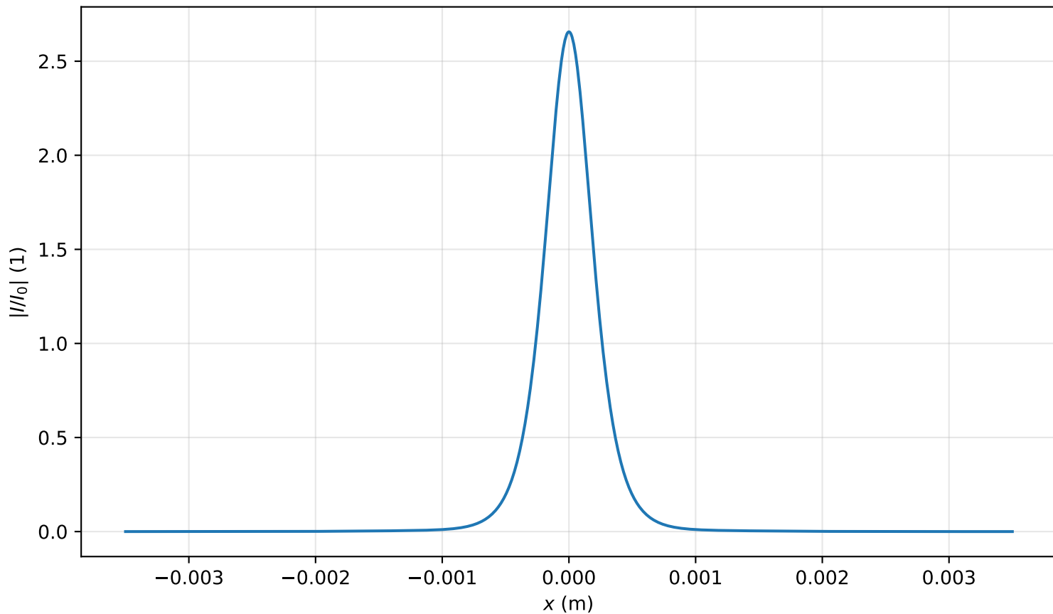
Intensity profile I(x, y = 0, z = 3.025m)/I_0 , P_{in}=1.0P_{cr} , artificial time
